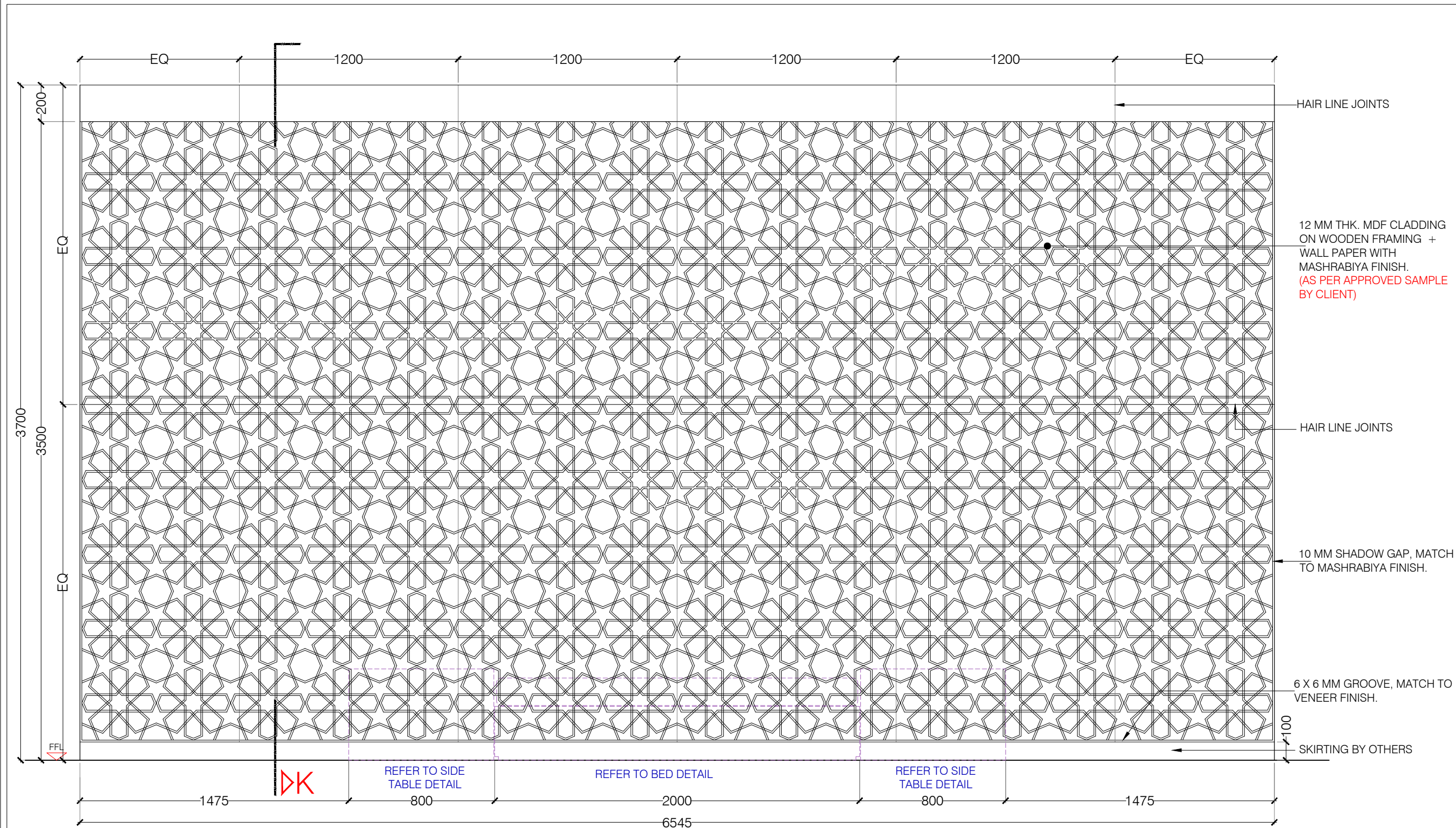
ELEVATION - A (BED ROOM - B)
